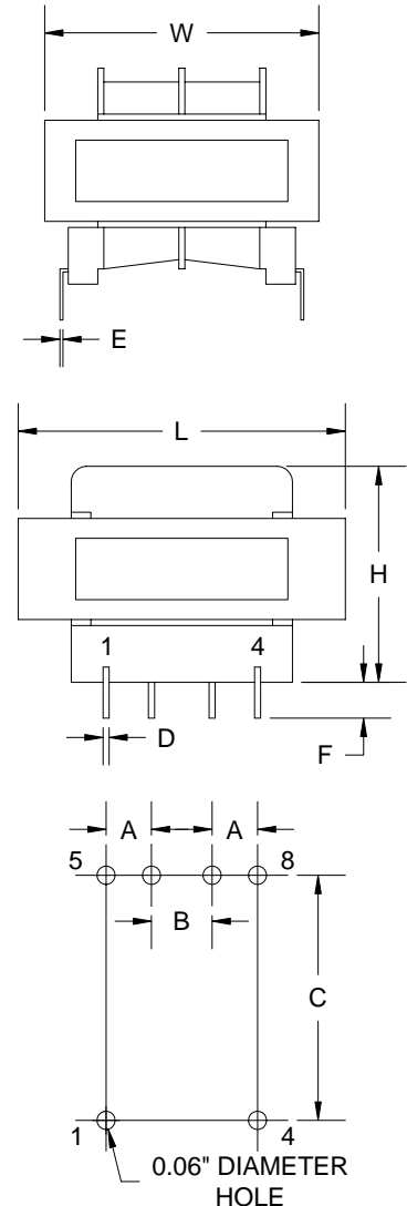
Board Layout
